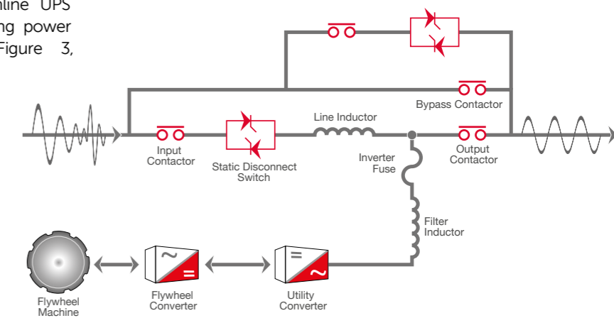
Figure 3. CLEANSOURCE® PLUS Parallel Online Architecture.
